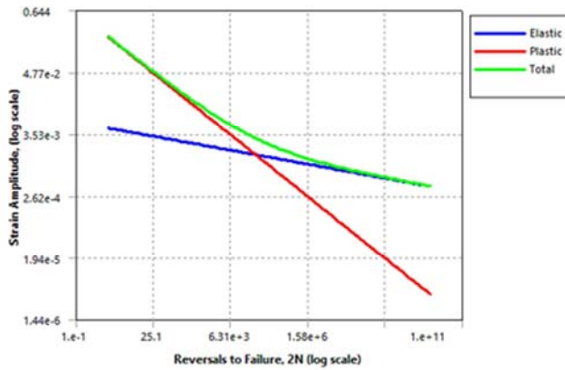
Figure 13. Structural Steel – strain life parameters.
