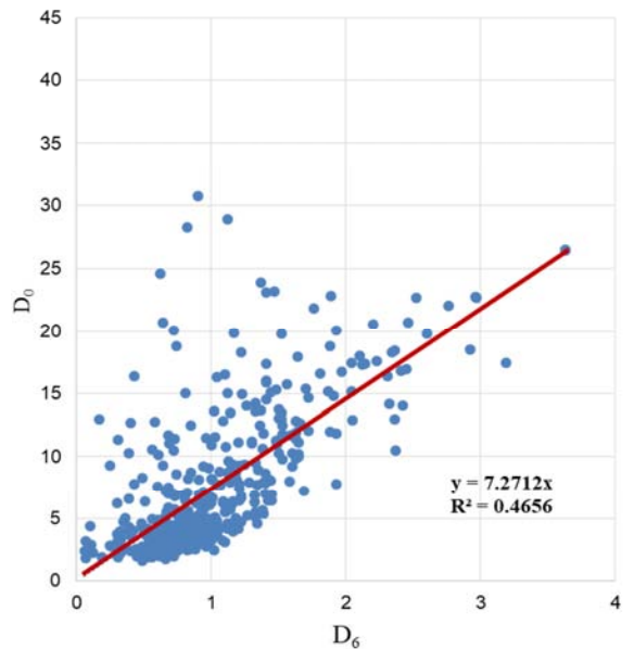
(b) D_0 vs D_6 Post-rehabilitation
