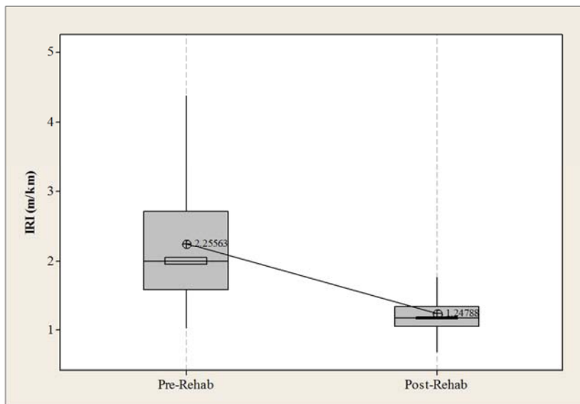
Figure 3. Comparative box-and-whisker plot of pre- and post-rehab IRI without and with CRM respectively.
