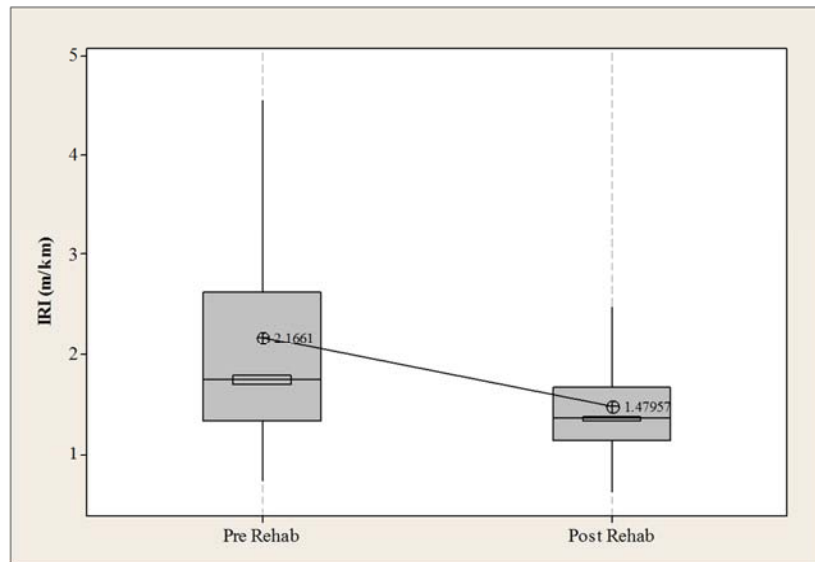
Figure 2. IRI before and after rehabilitation- SB&NB (truck lane).
