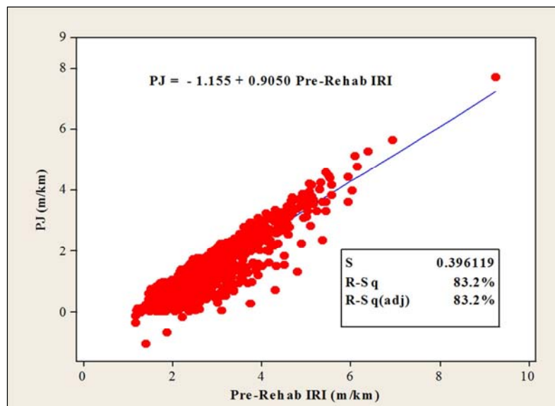
Figure 4. PJ (drop in IRI) with conventional AWC and CRM-SB.
