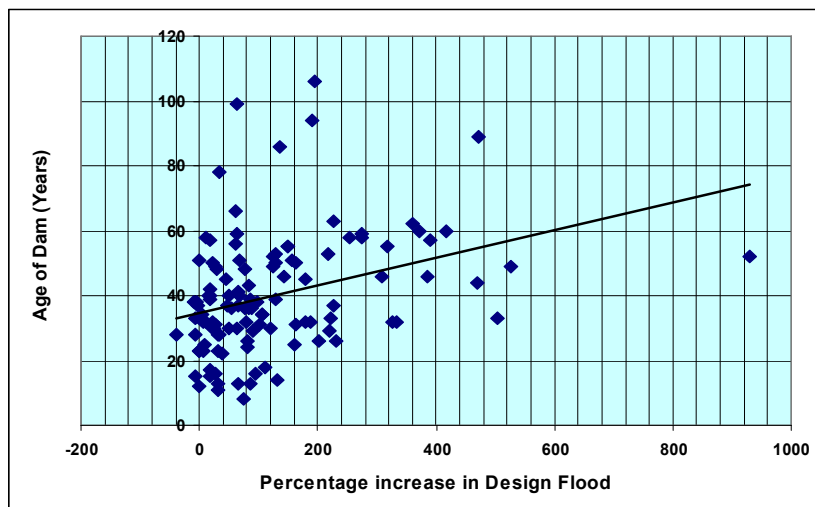
Figure 4. Scattered Plot of Increase in Design Flood Vs Age of Dam.
