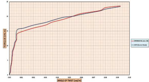
Figure (14). Experimental & ANSYS Torque – Twist curves for column specimen CFS-1
